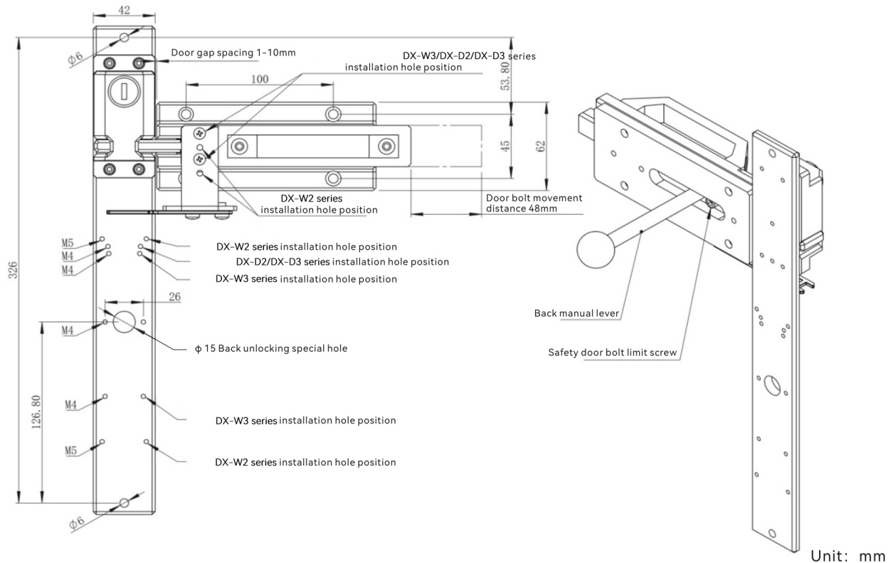
DXL-B-2 installation dimensions
