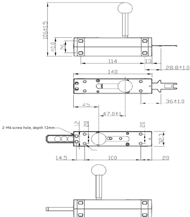
DXL-A-2 installation dimensions
