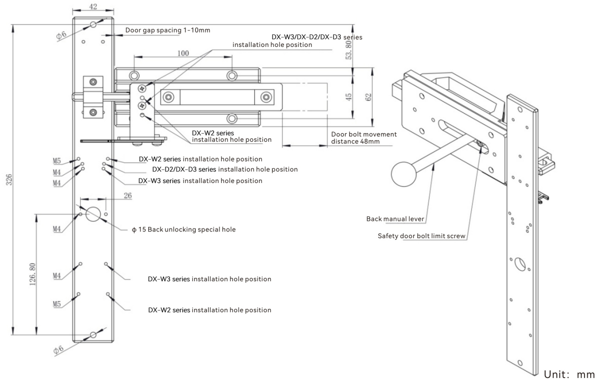
DXL-B-2 installation dimensions
