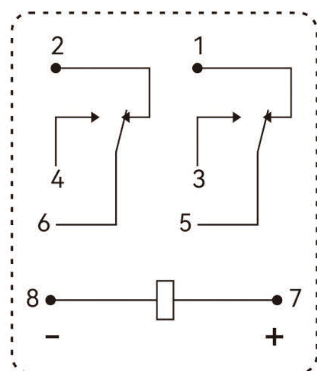
Circuit diagram
