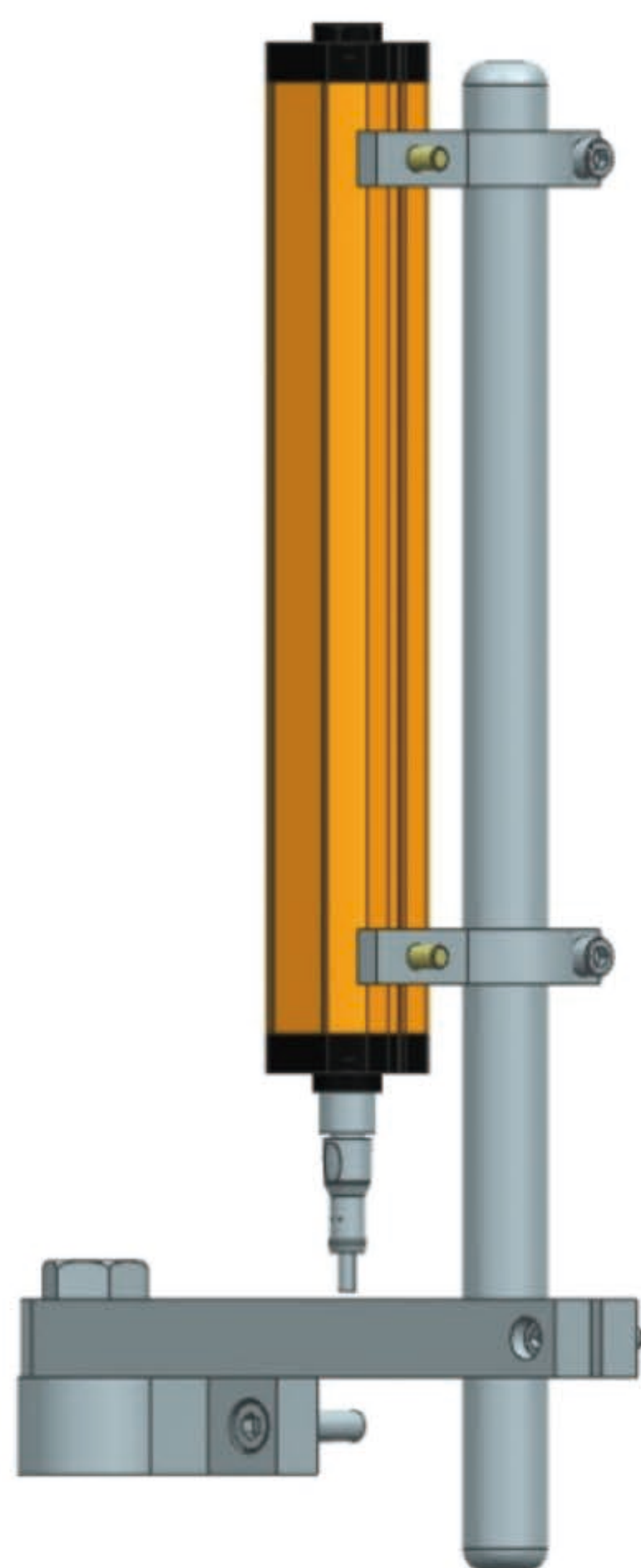
5. Stainless steel bracket installation (Order separately)
