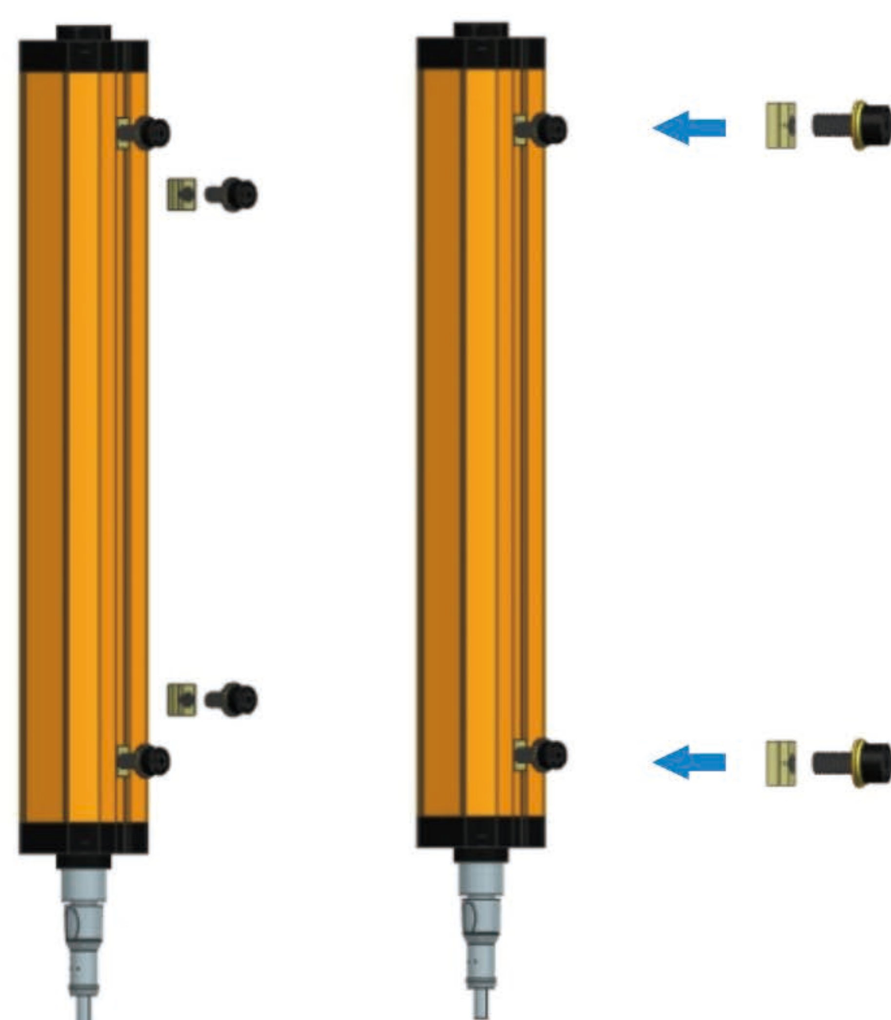
3. Installation method of convex nut (Optional accessories)
