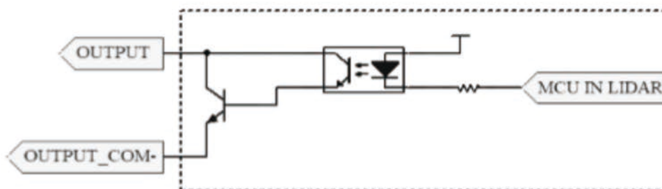
Figure 5-10 output circuit
