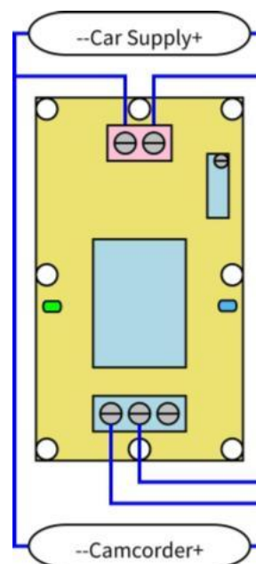
Figure 5-1 Typical Wiring Diagram of Application Cases
