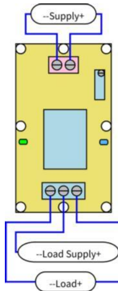
Figure 3-1 Typical Wiring Diagram of a Transistor Output Type Product
