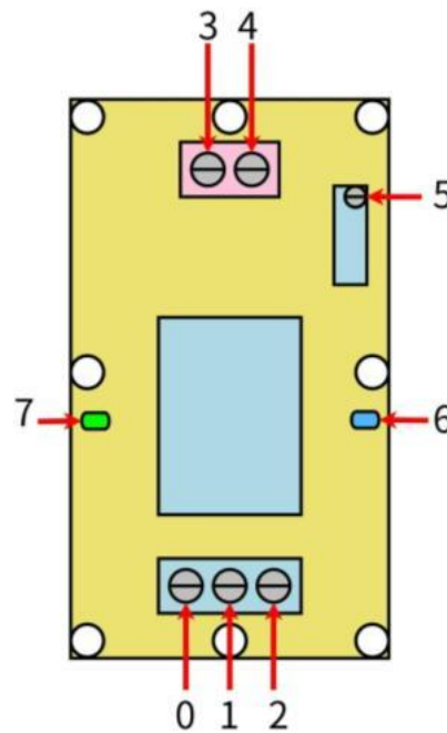
Figure 1-1 Product Front-side Marking Drawing
